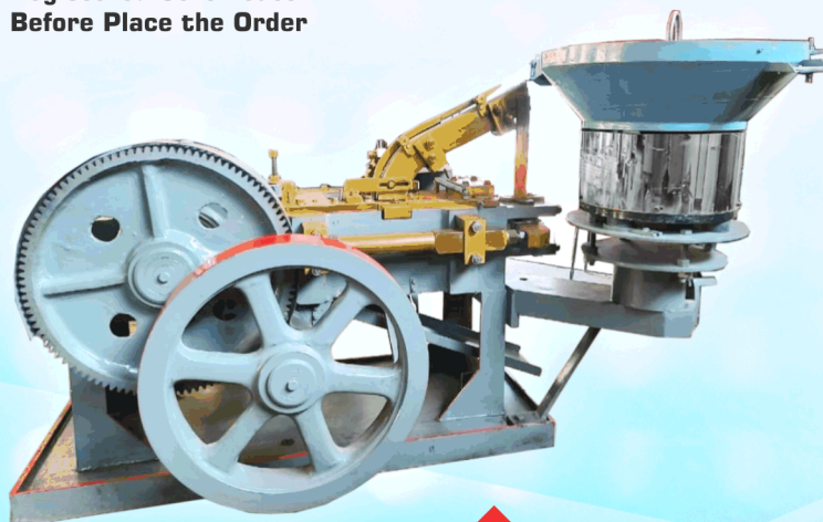
Fully Automatic Trimming Machine
